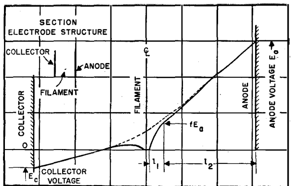
Fig. 7—Potential diagram for a plane plate structure. The dotted line represents the potential between filament strands; the full line indicates the potential in a plane containing the filament.
