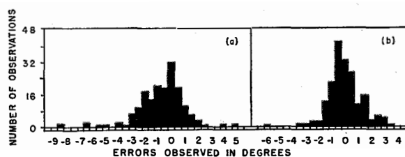
Fig. 19—Distribution of errors for field trials at Tangmere. (a) Manual direction-finder, Air Ministry Type 2A (169 observations). (b) Second experimental automatic direction-finder (186 observations).
