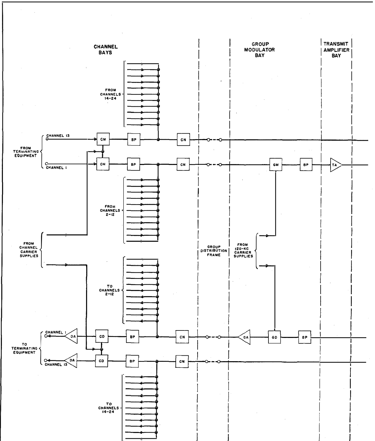
Fig. 2—Block diagram of transmission circuits for terminal and repeater. The letters in the boxes indicate the following: BP, Band-pass filter. CD, Channel demodulator. CM, Channel modulator. CN, Compensating network. DA, Demodulator amplifier. GA, Group amplifier. GD, Group demodulator. GM, group modu-
