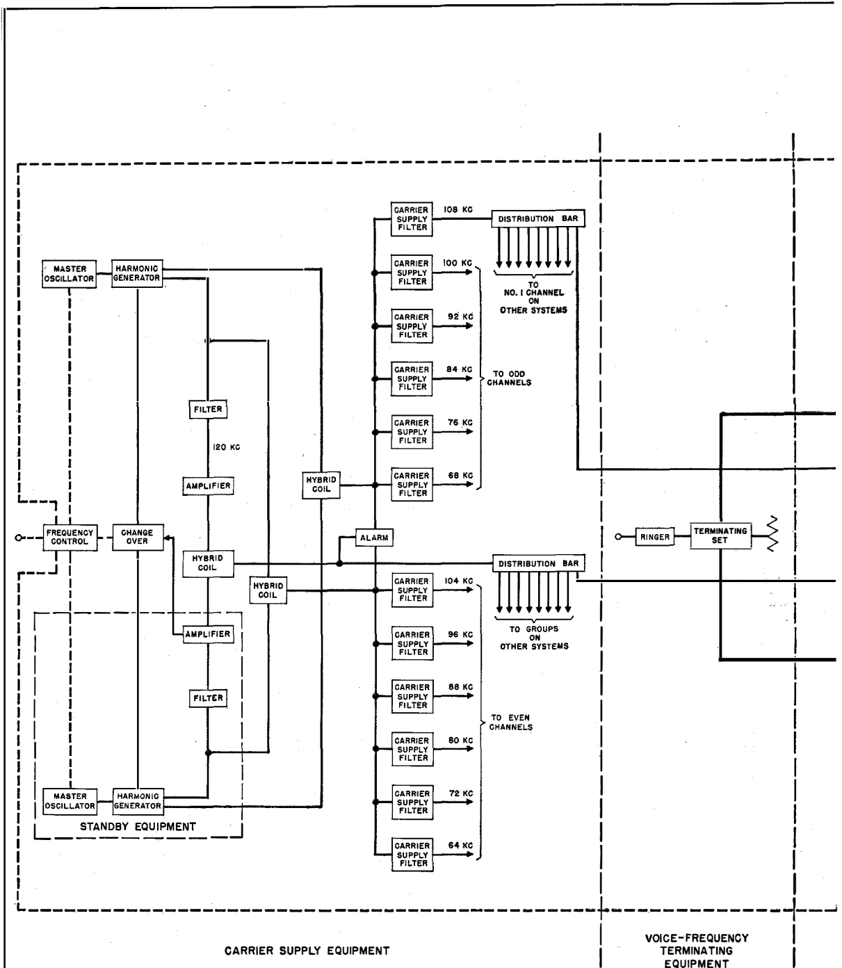
Fig. 1—Block diagram of 12-channel carrier-on-cable terminal equipment.
