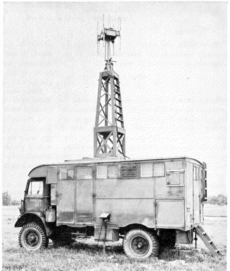
Fig. 2—Mobile direction-finder station.
