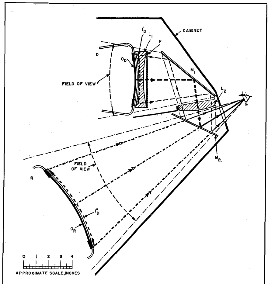
Fig. 21—Optical system of display unit DU74. D, direction-finder oscillograph. R, Radar oscillograph. L_1 , Correcting lens. F, Blue colour filter. M_1 , Polished steel reflector. L_2 , Magnifying lens. M_2 , Plate-glass reflector incorporating yellow colour filter. O_D , direction-finder trace. I_D' , Intermediate image of O_D , curvature corrected. I_D'' , Final image of O_D . O_R , Radar image. ( I_D' is normally adjusted to coincide with O_R .)
