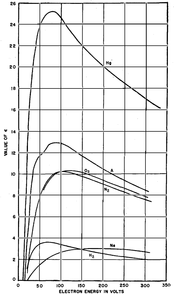
Fig. 5—The efficiency of ionization \epsilon of several gases as a function of electron energy. See Table 2.
