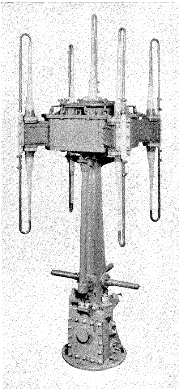
Fig. 5—FV5 antenna system.
