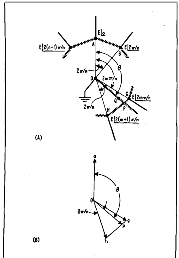
Fig. 8—Principle of linear phase shifter. (A) Polygonal arrangement of n resistance elements. (B) Vector diagram.
