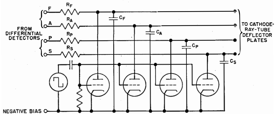
Fig. 10—Converter circuit.
