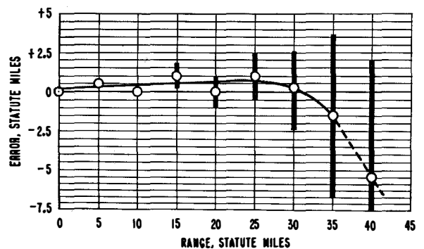
Fig. 7—Range test on an aircraft at a height of 2000 feet. f_1 = 100.8 megacycles, f_2 = 110 megacycles.
