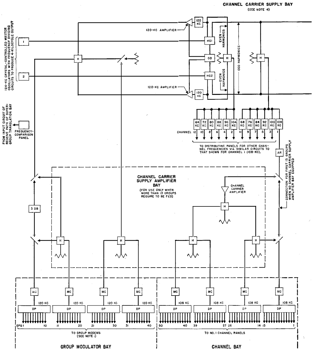
Fig. 5—Block diagram of carrier supply. The letters in the boxes indicate the following: AR, Adjusting resistance. CO, Change-over (switching) panel. DB, Resistance pad of indicated attenuation in decibels. DP, Distributing panel. GP, Group. H, Hybrid coil. HG, Harmonic generator. KC, Band-pass filter of indicated midband frequency in kilocycles per second. MC, Matching coil. S/GP, Supergroup.
