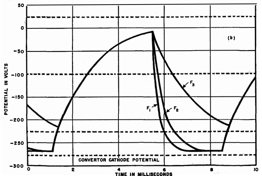
Fig. 11—(a) Converter input potentials and corresponding output waveforms for bearing 000 degrees. (b) Repeater output waveforms for various cable time-constants. The waveforms in (b) correspond with F in (a), and the following time-constants: F_1 —0.25 millisecond, F_2 —0.5 millisecond, F_3 —2.0 milliseconds.
