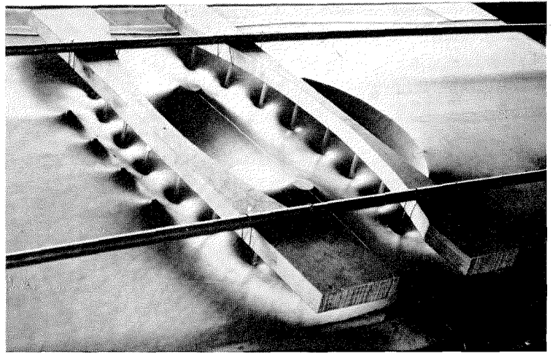
Fig. 6—Rubber-table model of a structure similar to KM2 of Fig. 3. The filaments appear on the left side and the collector on the right.
