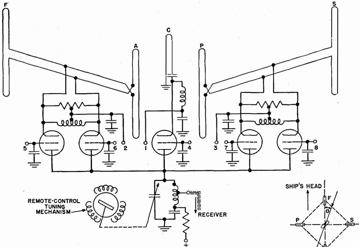
Fig. 7—Circuit of FV5 antenna system. Key to interconnection with direction-finder office equipment: (1) To fixed cathode resistance. (2, 3) To differential variable cathode resistances. (4) From ground (normal operation), or from calibrator (modulation test). (5, 6) From 5 kilocycle-per-second oscillator. (7, 8) From 6 kilocycle-per-second oscillator.
