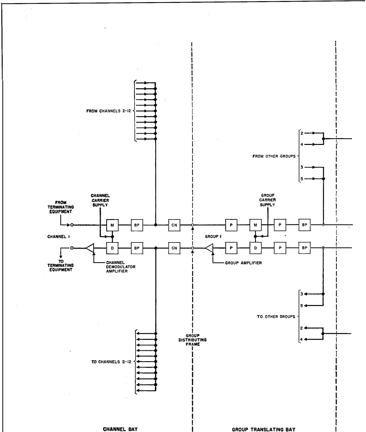
Fig. 4—Block diagram of terminal equipment, excluding terminal repeaters. The letters in the boxes indicate the following: C, Combining panel. BP, Band-pass filter. CN, Compensating network. D, Demodulator. HP, High-pass filter. LP, Low-pass filter. M, Modulator. P, Resistance pad.
